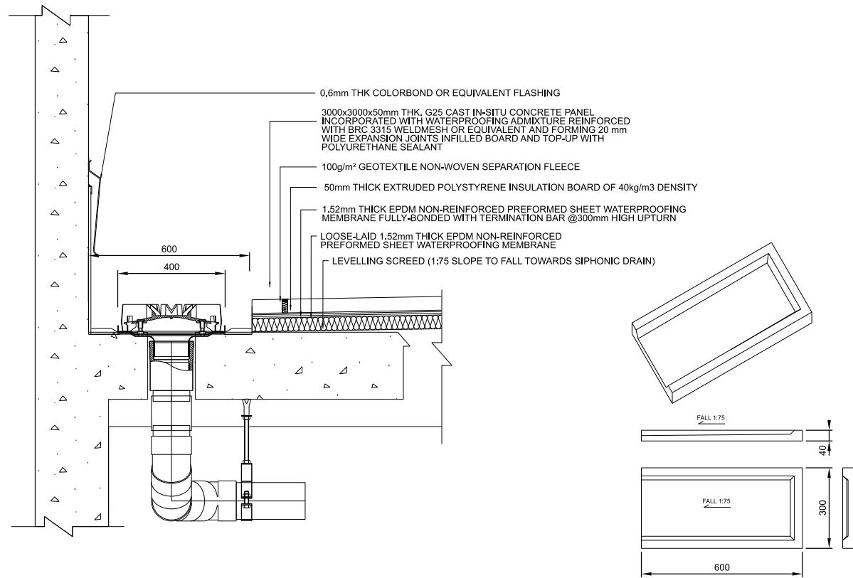
TYP. WATERPROOFING DETAIL - SECTION A1-A1 SIPHONIC OUTLET ON RC ROOF NEAR PARAPET WALL 1:10
