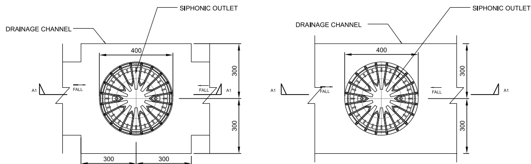
TYPE-1 LOCALISED POCKET SCUPPER DETAIL 1:10
