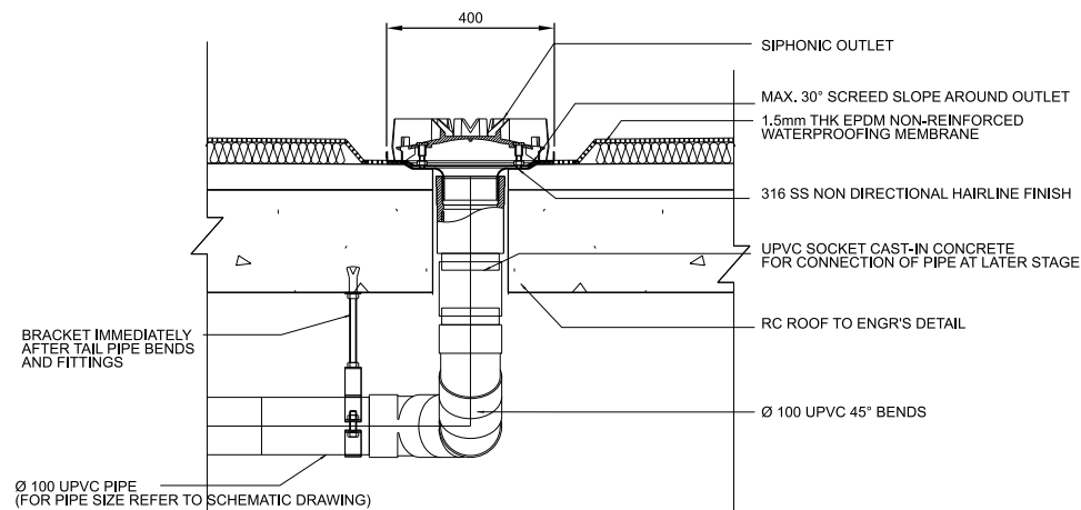
TYP. WATERPROOFING DETAIL - SECTION A1-A1 SIPHONIC OUTLET ON RC ROOF 1:10
