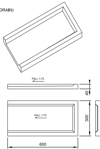
CONCRETE SPLASH BLOCK NTS
